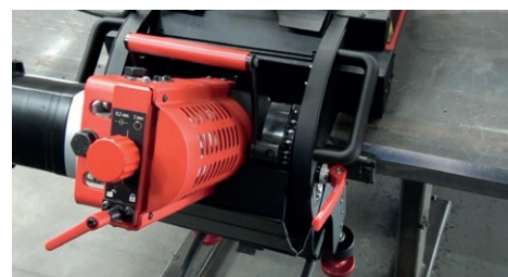
Innovative and ergonomic bevel angle adjustment system with release lever requires no additional tools
