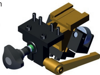
Small clamp for bulb profiles 50 – 180 mm (option) DCS-0824-0037-02-0
