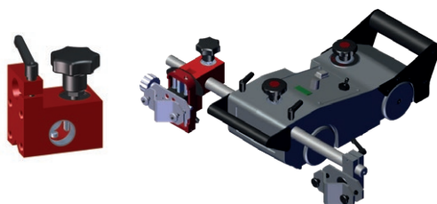
Sliding clamping block type 2 UCW-0475-15-00-00-1
