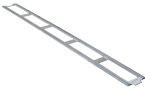
Track Assembly 1800 mm (70,9") „V” Groove Center Line 152 mm (6") TRO-0475-13-00-00-0
